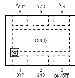
6-Lead LLP Package (LD)
