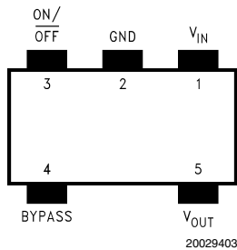
5-Lead Small Outline Package (M5)
