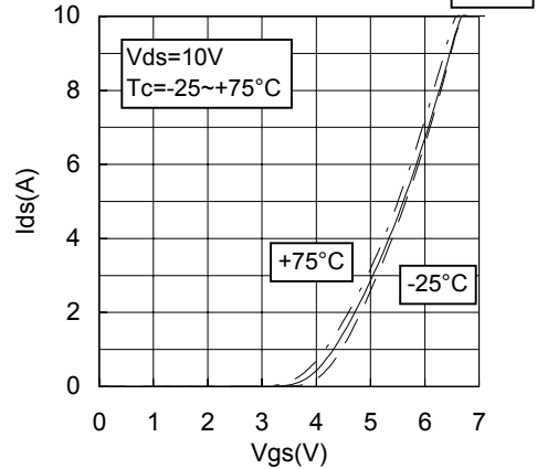
Vgs-Ids CHARACTERISTICS 2
