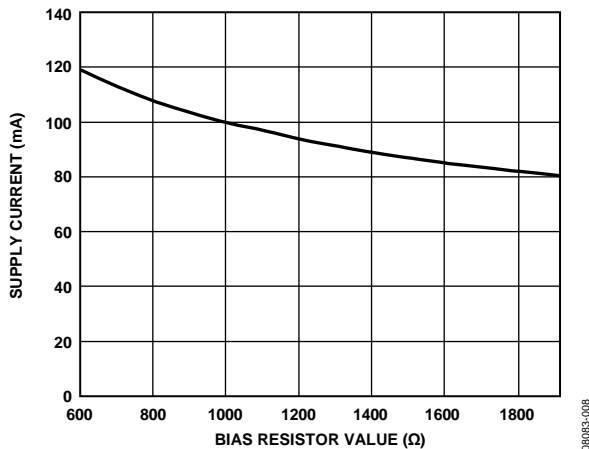
Figure 39. LO Supply Current vs. LO Bias Resistor Value
